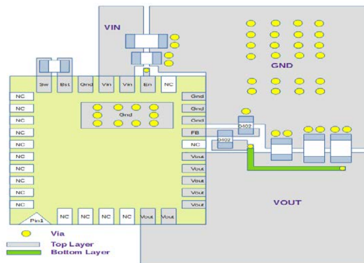
Figure 6: Recommended PCB Layout
