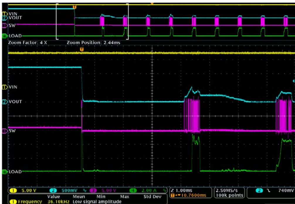
Short Circuit RESPONSE, 12V Vin, 1.2V Vout
