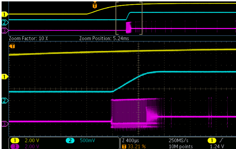
Pre-bias start up (~400mV), 12V Vin, 1.2V Vout (Ch2), SW (Ch3), Vin(Ch1)
