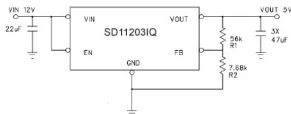
Figure 1: Simplified Applications Circuit
