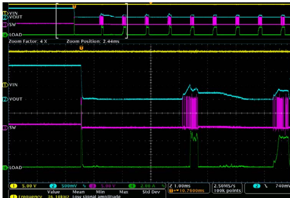
Short Circuit RESPONSE, 5V Vin, 1.2V Vout
