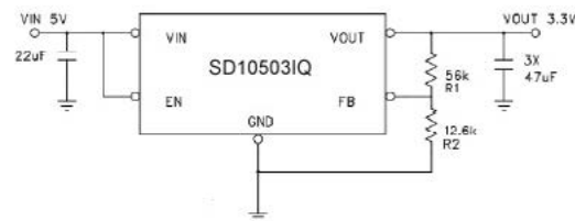
Figure 1: Simplified Applications Circuit
