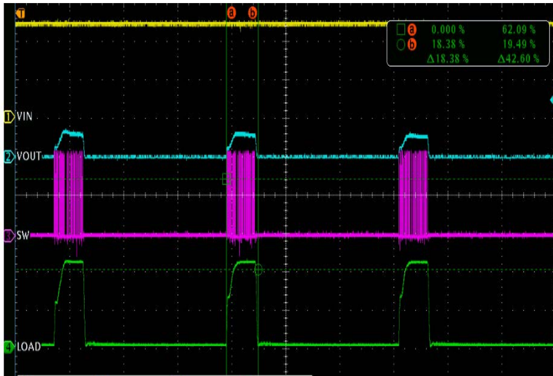
Short Circuit RECOVERY, 5V Vin, 1.2V Vout
