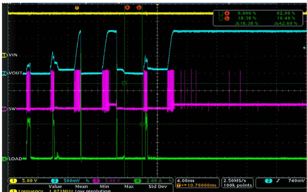
Short Circuit Hiccup Mode, 5V Vin, 1.2V Vout
