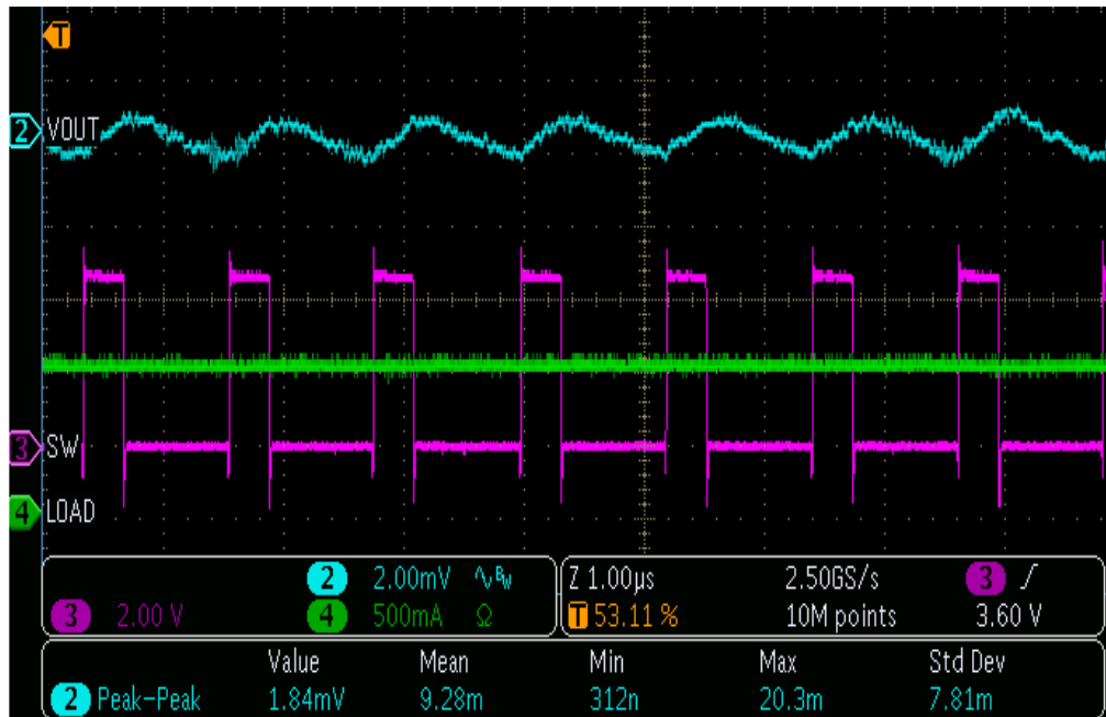
OUTPUT Ripple, 5V Vin, 1.2V Vout, 1A DC LOAD
