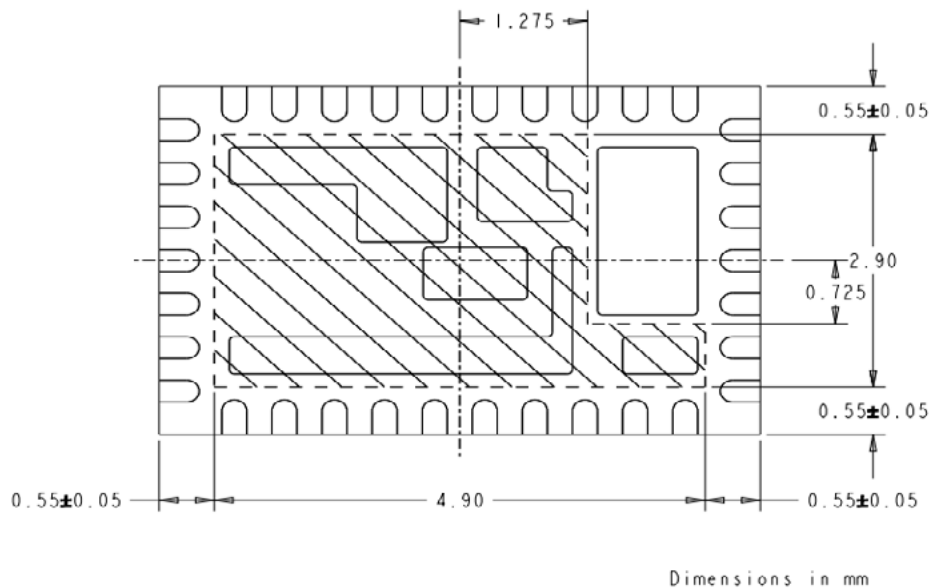
Figure 7: Lead-Frame exposed metal (Bottom View)
