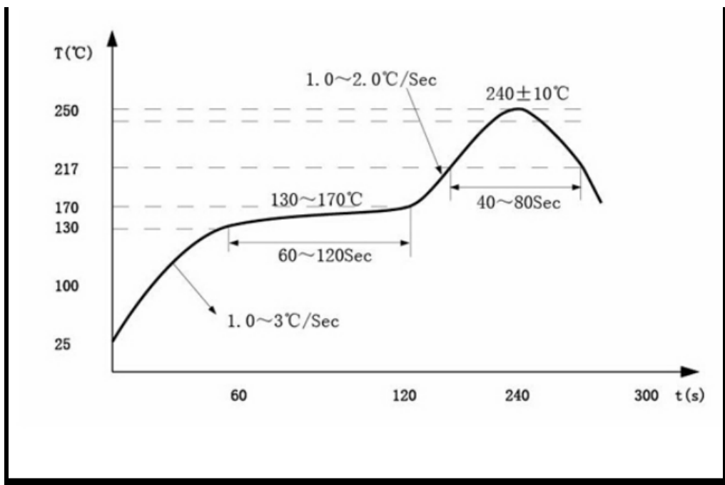
Figure 5: IR Reflow Profile for the 6x4 QFN Package
